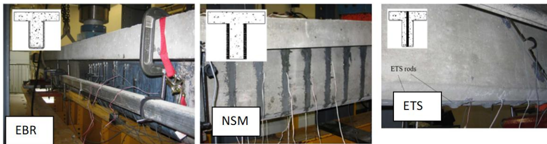
Figure 1. Design of shear strengthening using FRP bars/sheets in a) EBR b) NSM c) ETS [60]
