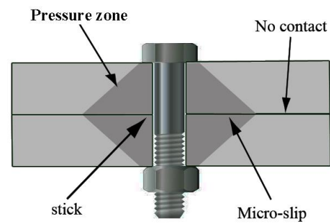
Figure (2): The micro-slip at the jointed interface
