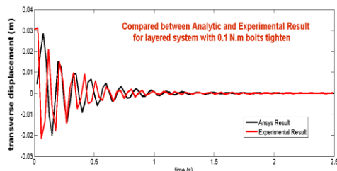
Figure (12): The displacement diagram at 0.1 N.m bolts tighten
