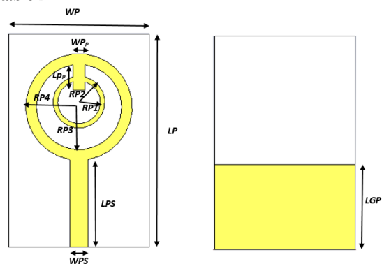
Figure (5): Front and back view of Ant III
