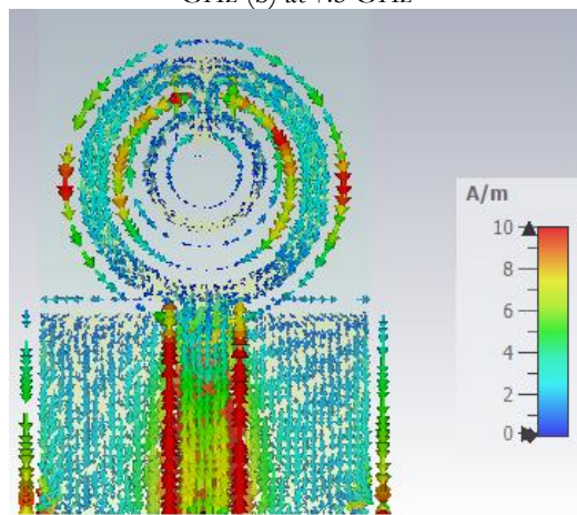
Figure (11): The surface current at 2.56 GH
