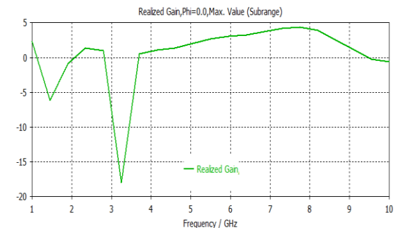
Figure (9): The realized gain of the Ant III
