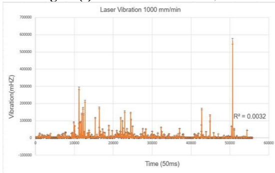
Figure (4): Laser vibration 1000mm/min.
